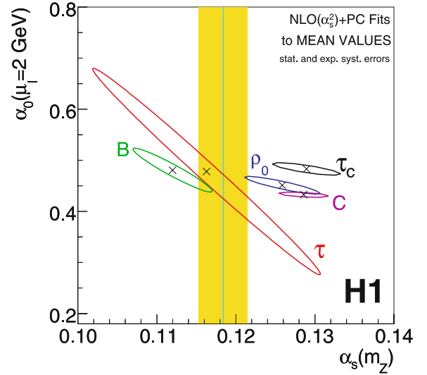
Fig. 7. Results of fits to the mean values of \tau , B , \rho_0 , \tau_C and the C -parameter in the (\alpha_s, \alpha_0) plane. The 1\sigma contours correspond to \chi^2 = \chi^2_{\min} + 1 , including statistical and experimental systematic uncertainties. The value of \alpha_s ( vertical line ) and its uncertainty ( shaded band ) are taken from [35]. Note the enlarged scale compared to Fig. 4
