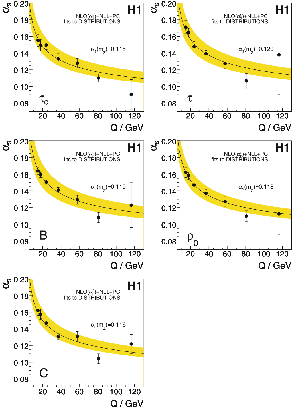
Fig. 5. The strong coupling \alpha_s as a function of the scale Q . The individual fit results, shown as points with error bars , are obtained from fits to the differential distributions in \tau_C , \tau , B , \rho_0 and C within each Q bin. The errors represent the total experimental uncertainties. For each event shape observable a value of \alpha_s(m_Z) is indicated in the plot, determined from a fit to the \alpha_s(Q) results using the QCD renormalisation group equation. The corresponding fit curves are shown as full lines . The shaded bands represent the uncertainties on \alpha_s(Q) from renormalisation scale variations
