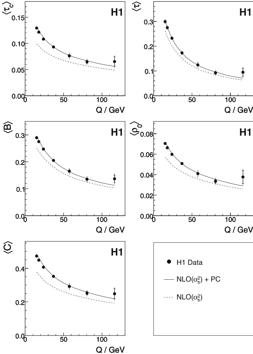
Fig. 3. Mean values of event shape variables corrected to the hadron level as a function of the scale Q . The data, presented with statistical errors ( inner bars ) and total errors ( outer bars ), are compared with the results of NLO QCD fits including power corrections (PC). The dashed curves show the NLO QCD contribution to the fits
