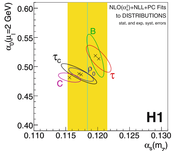
Fig. 4. Fit results to the differential distributions of \tau , B , \rho_0 , \tau_C and the C -parameter in the (\alpha_s, \alpha_0) plane. The 1\sigma contours correspond to \chi^2 = \chi_{\text{min}}^2 + 1 , including statistical and experimental systematic uncertainties. The value of \alpha_s (vertical line) and its uncertainty (shaded band) are taken from [35]
