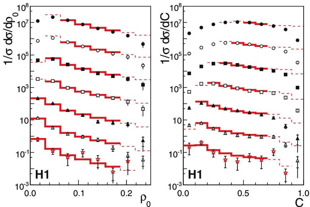
Fig. 2. Normalised event shape distributions corrected to the hadron level for \rho_0 and the C -parameter. The data are presented with statistical errors ( inner bars ) and total errors ( outer bars ). The measurements are compared with fits based on a NLO QCD calculation including resummation (NLL) and supplemented by power corrections (PC). The fit results are shown as solid lines and are extended as dashed lines to those data points which are not included in the QCD fit (see Sect. 5.3). The symbols and scale factors are defined in Fig. 1
