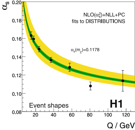
Fig. 6. The strong coupling \alpha_s as a function of the scale Q from an average of the results obtained by fitting the differential event shape distributions. The errors represent the total experimental uncertainties. A value of \alpha_s(m_Z) is indicated in the plot, determined from a fit to the \alpha_s(Q) results using the QCD renormalisation group equation. The fit curve is shown as the full line . The inner (outer) shaded band represents the uncertainty of the fitted \alpha_s(Q) from experimental errors (the renormalisation scale variation)
