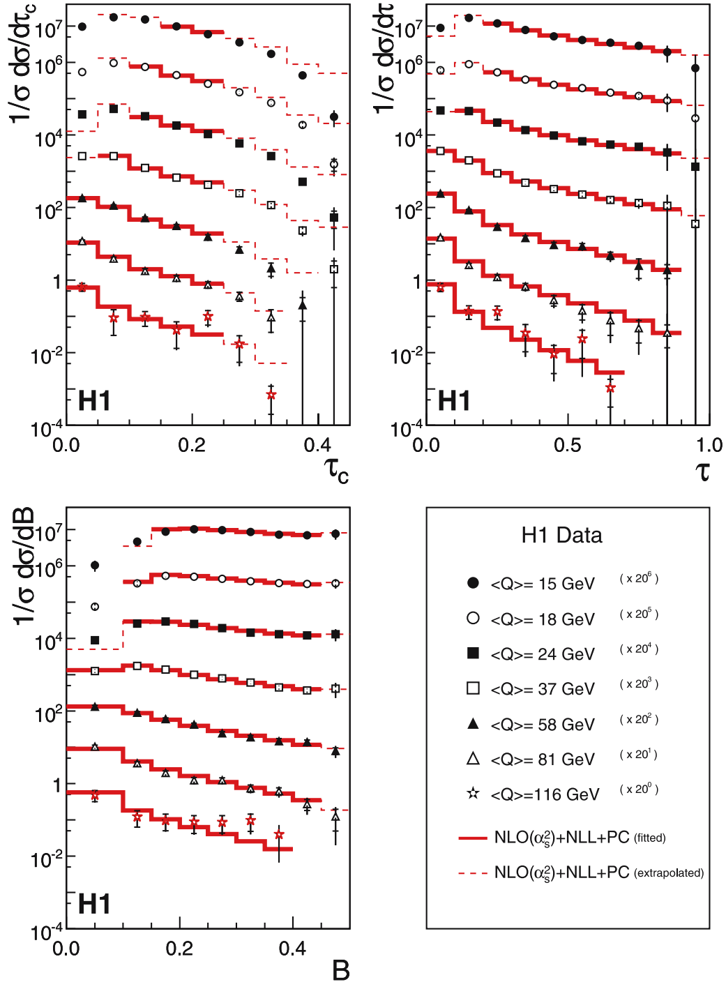
Fig. 1. Normalised event shape distributions corrected to the hadron level for \tau_C , \tau and B . The data are presented with statistical errors ( inner bars ) and total errors ( outer bars ). The measurements are compared with fits based on a NLO QCD calculation including resummation (NLL) and supplemented by power corrections (PC). The fit results are shown as solid lines and are extended as dashed lines to those data points which are not included in the QCD fit (see Sect. 5.3)
